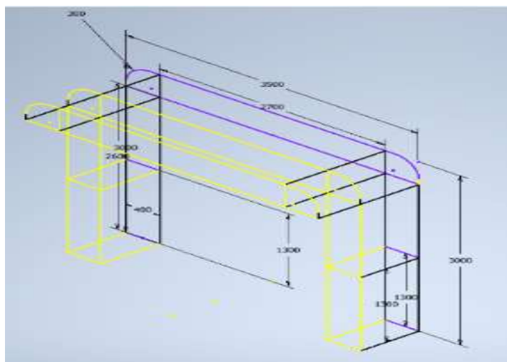
Gambar 1. Desain 2D sketch
